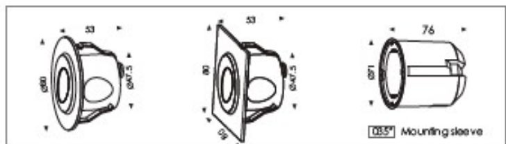
Installation with clips embedded into sleeve, fix on the concrete wall
