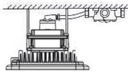
E. U-Bracket Mounting
